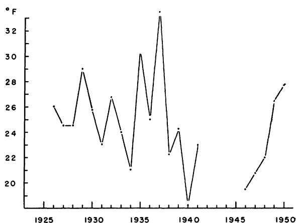
FIG. 2. Mean midwinter temperatures on St. Paul Island, 1926-50. (January, February, and March; from Table 2.)
